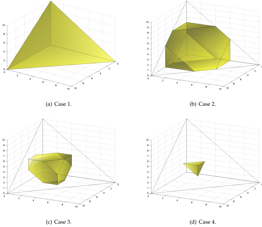
Fig. 1: n = 4 , core covers of cases 1, 2, 3, and 4.
