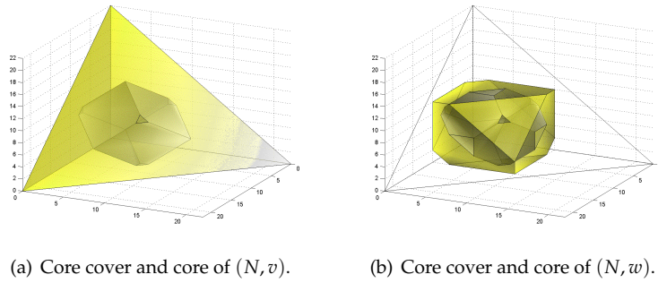
Fig. 2: Core cover contains the core.
