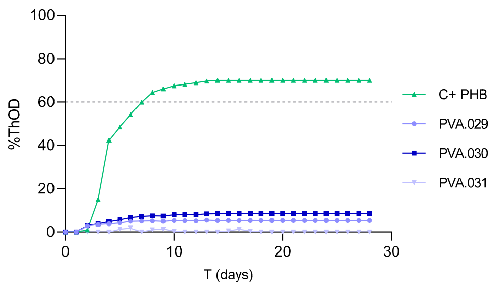
Figure 1. Biodegradation expressed by %ThOD for the different materials and the positive control (C+ PHB). Discontinuous line: 60% biodegradability threshold.
