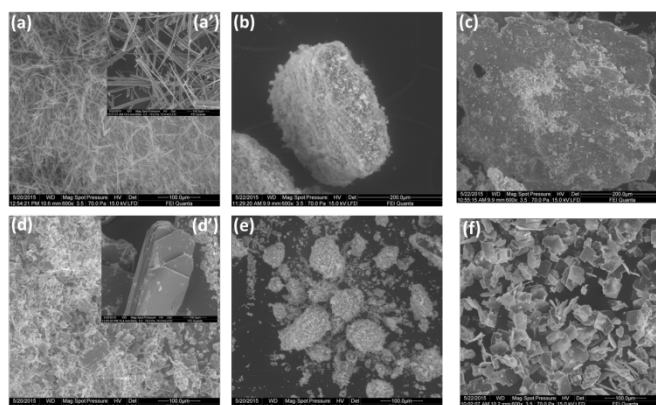
Figure 1. SEM images X600 of (a) [Zn(ibu) 2 (SCS)] ( 1 ) and (d) [ZnCl(ibu)(SCS)] ( 2 ) with their respective single crystals (a' and d'); post-treatment materials; (b) ( 1 ) at pH = 5; (e) ( 2 ) at pH = 5; (c) product after anionic exchange in PBS solution, (f) ( 2 ) in an aqueous environment.
