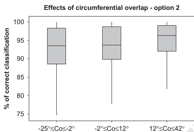
Fig. 10. Effects of circumferential overlapping ( option 2 ).
