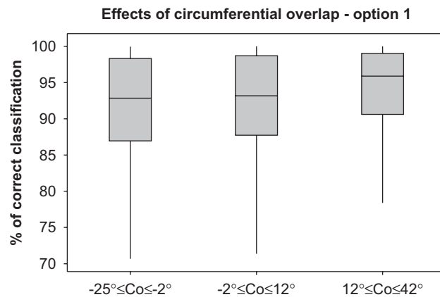
Fig. 6. Effects of circumferential overlapping (option 1).
